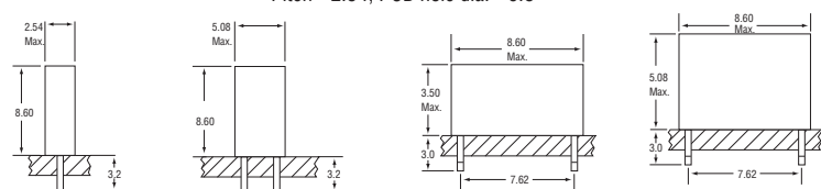
Pitch=2.54, PCB hole dia.=0.8
