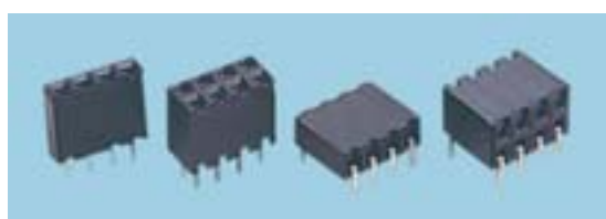
Pitch=2.54, PCB hole dia.=0.8
